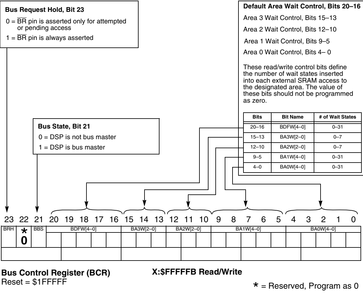
Figure B-5. Bus Control Register (BCR)
