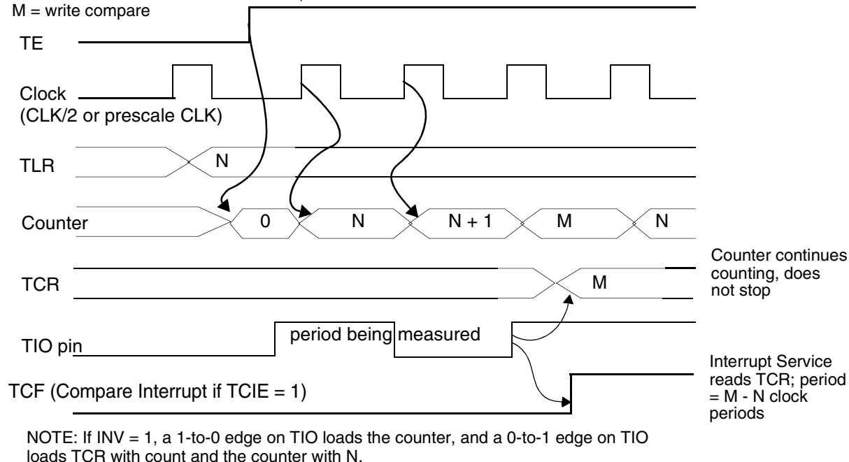
Figure 9-13. Period Measurement Mode, TRM = 1
