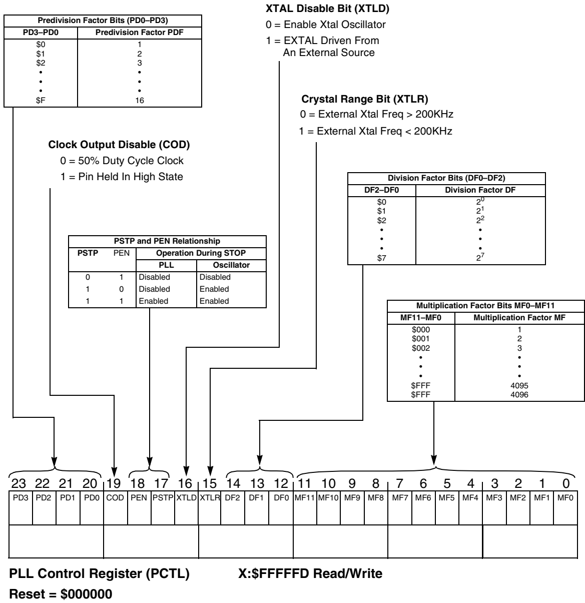
Figure B-4. Phase-Locked Loop Control Register (PCTL)
