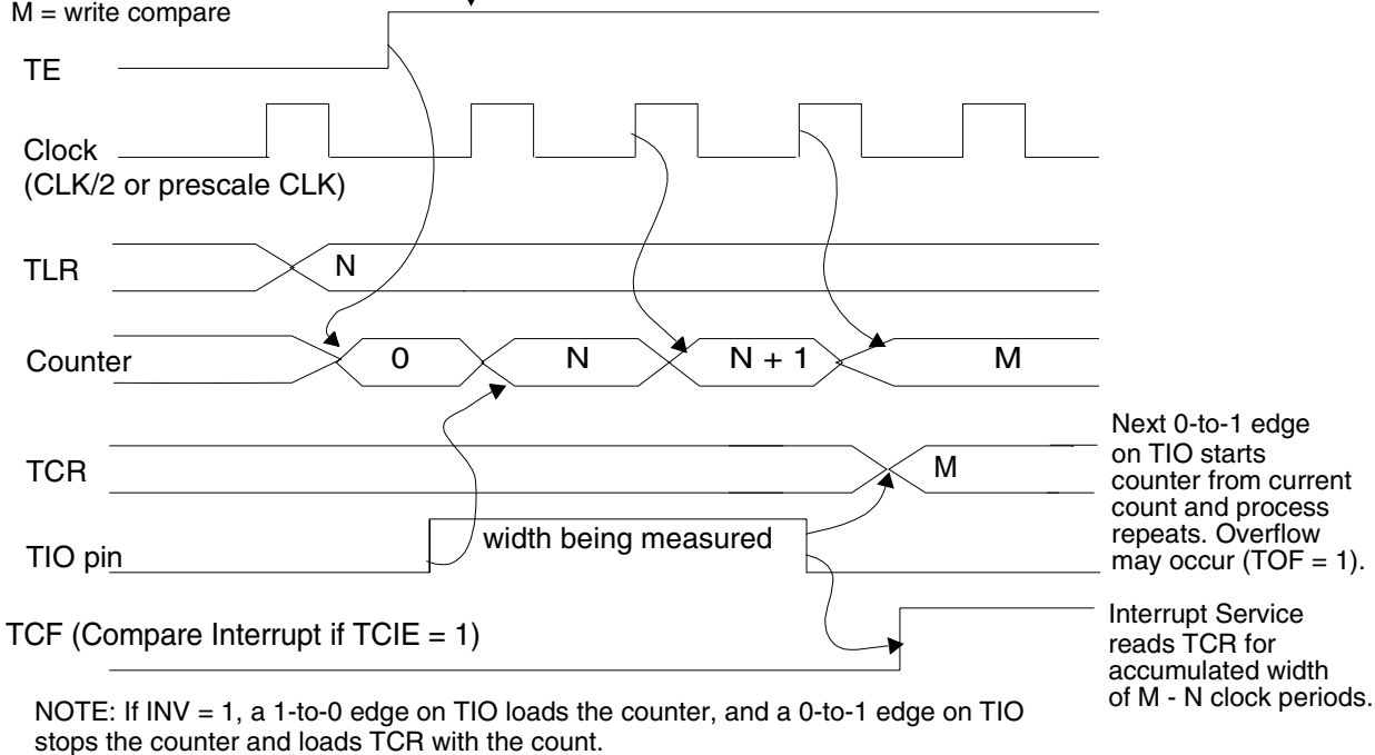
Figure 9-12. Pulse Width Measurement Mode, TRM = 0
