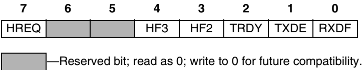
Figure 6-17. Interface Status Register (ISR)
