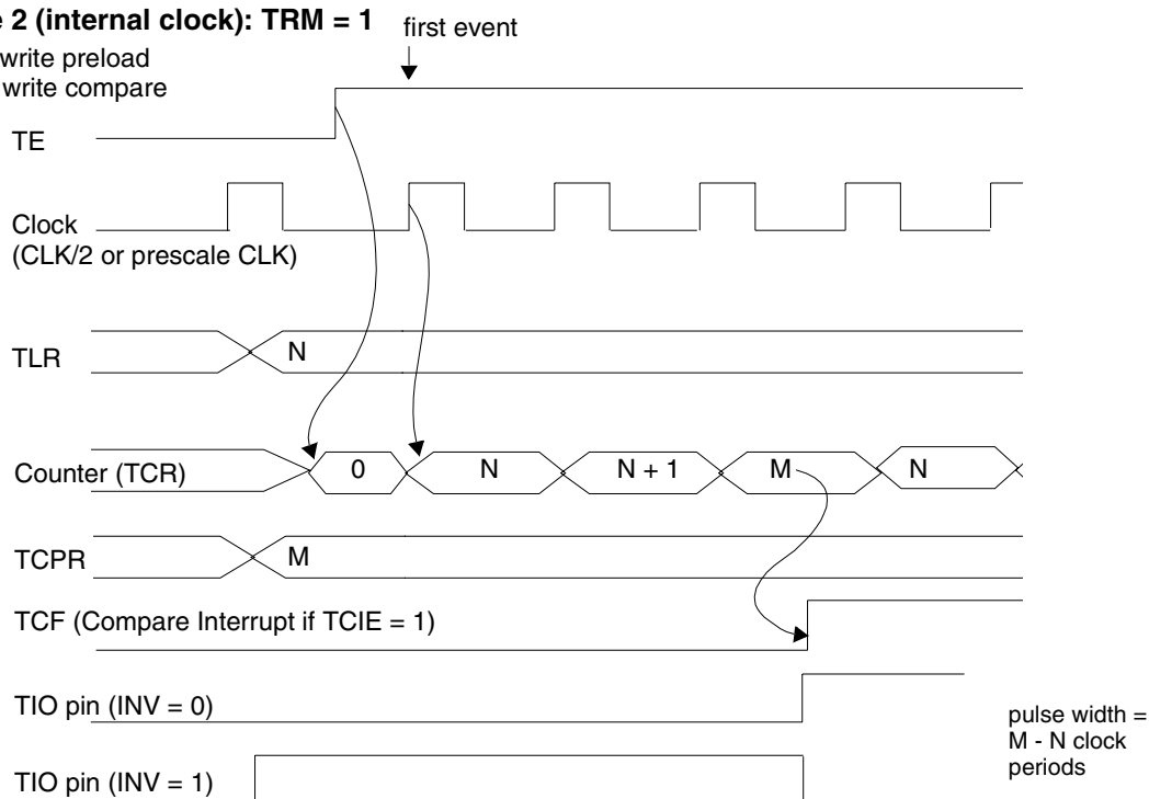
Figure 9-7. Toggle Mode, TRM = 1
