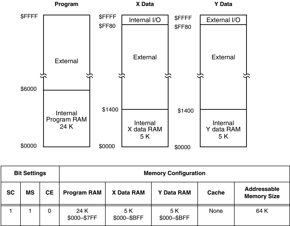
Figure 3-7. 16-bit Space with Switched Program RAM (1, 1, 0)
