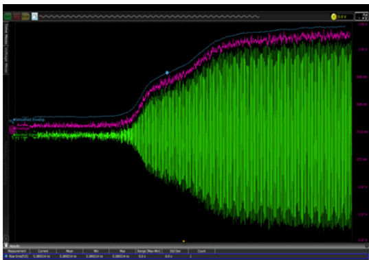
Amplitude demodulation.
