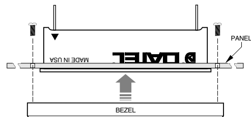
RETAINING CLIP INSTALLATION
