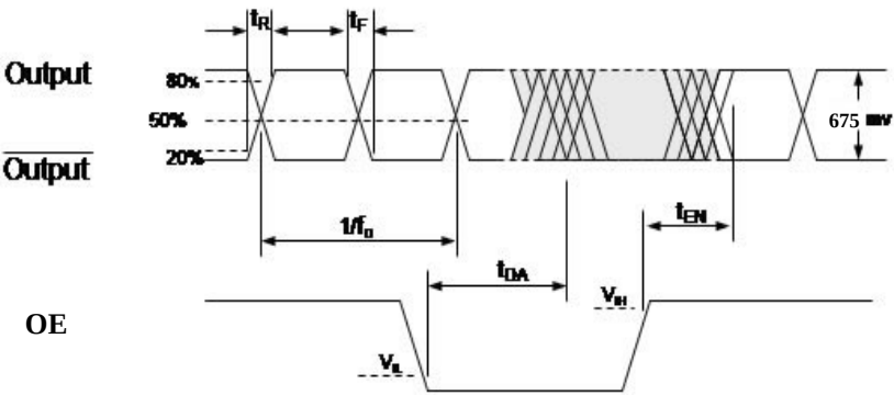
Figure 2. HCSL Output Waveform
