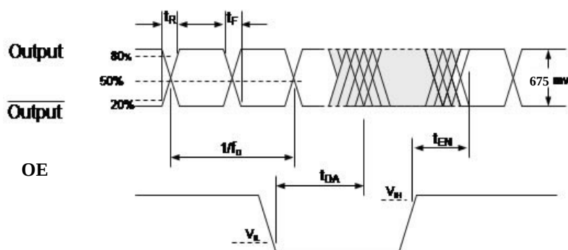
Figure 3. HCSL Output Waveform
