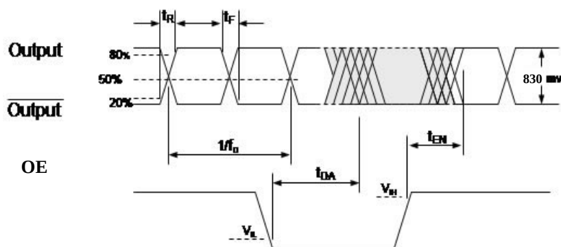
Figure 4. LVPECL Output Waveform
