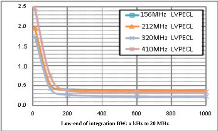
Figure 2. LVPECL Phase Jitter (integrated phase noise)
