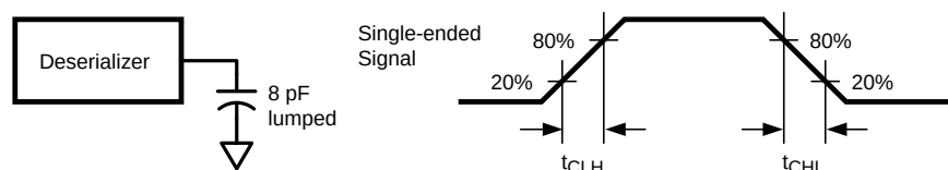
Figure 11. Deserializer LVCMOS/LVTTL Output Load and Transition Times
