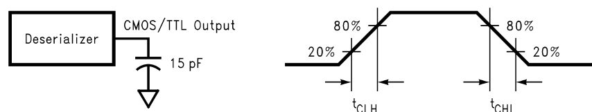
Figure 5. Deserializer CMOS/TTL Output Load and Transition Times
