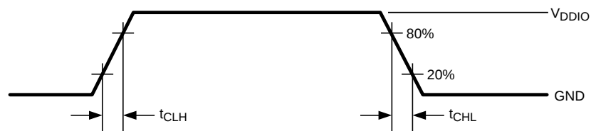
Figure 3. LVCMOS Transition Times
