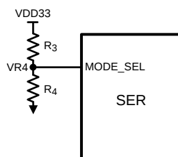
Figure 16. MODE_SEL Connection Diagram
