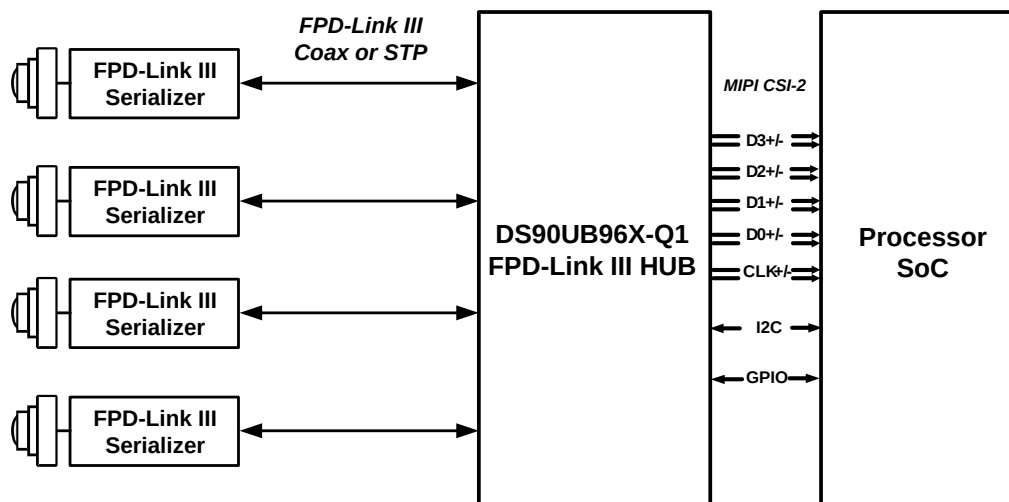
Figure 1-1. Applications Diagram
