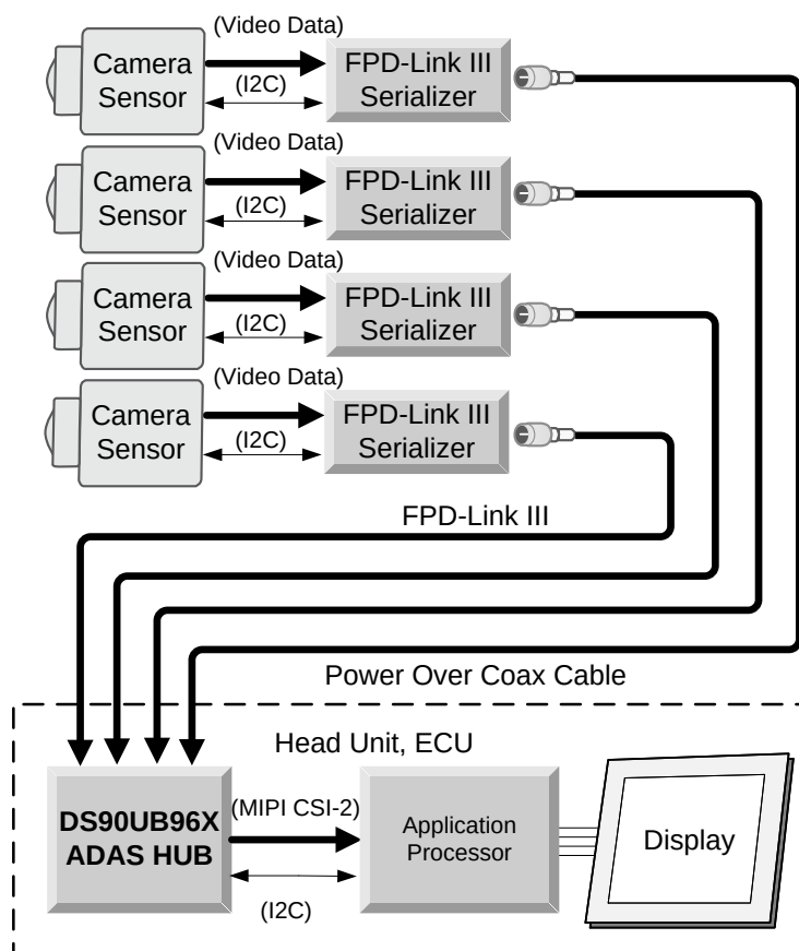
Figure 1-2. Typical Configuration
