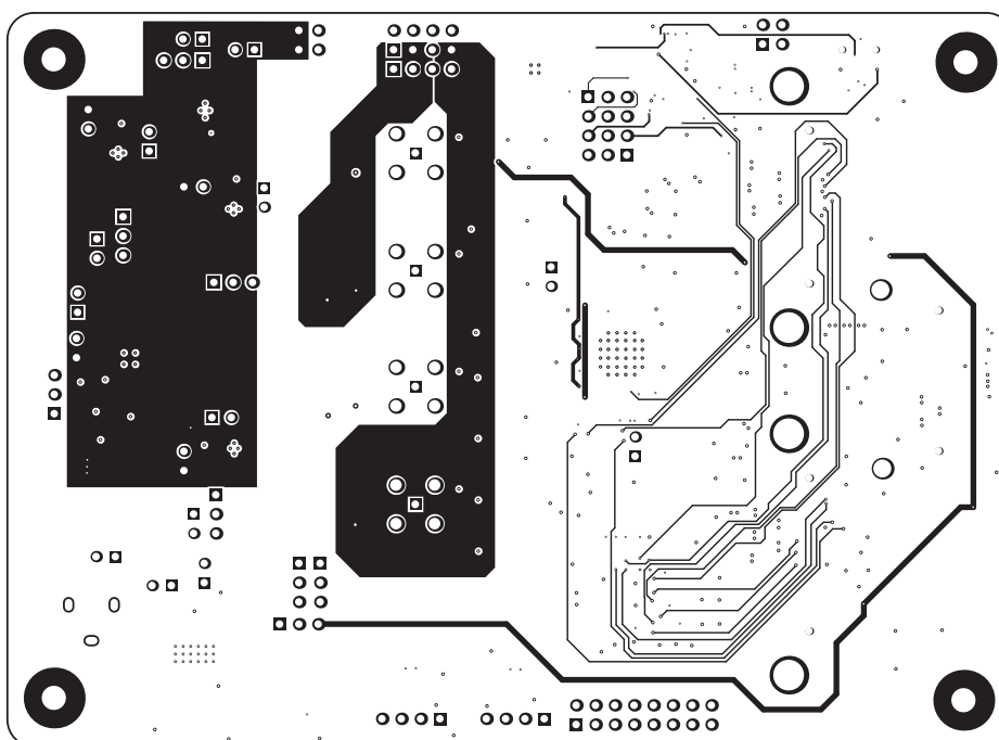
Figure 3-5. Layer 3
