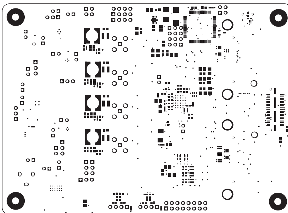
Figure 3-9. Bottom solder
