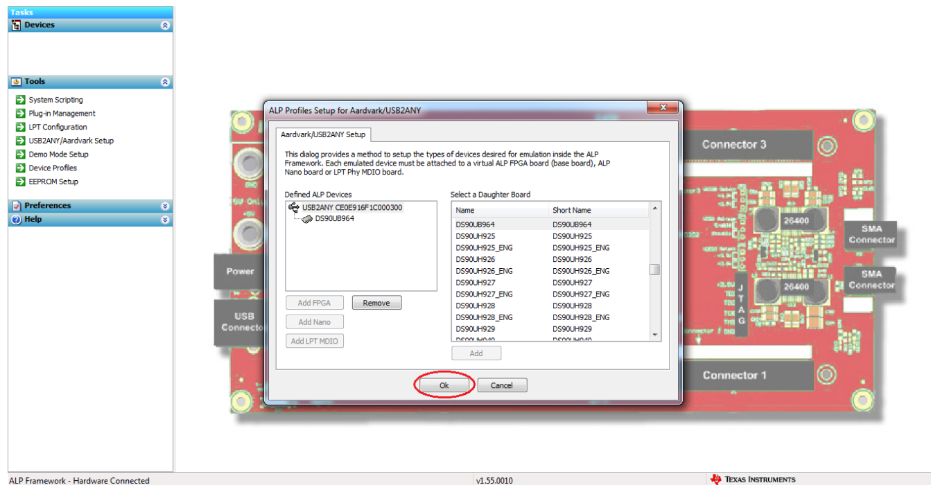
Figure 1-16. Finish Setup
