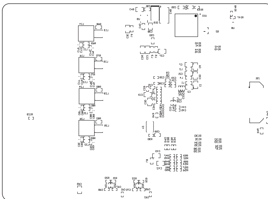
Figure 3-10. Bottom Overlay
