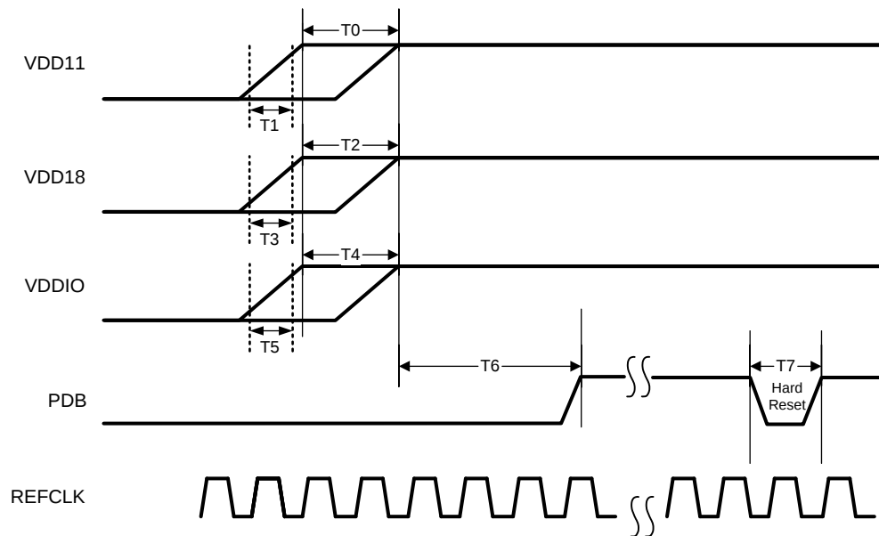
Figure 45. Power-Up Sequencing
