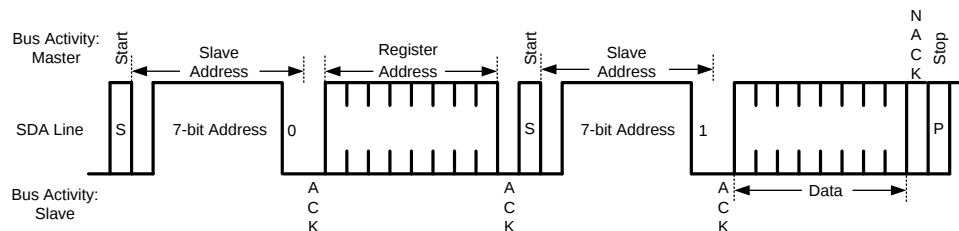
Figure 35. Serial Control Bus — READ
