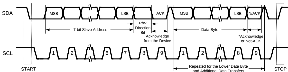
Figure 37. Basic Operation
