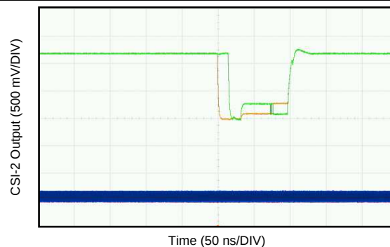
Figure 42. CSI-2 DATA and Continuous CLK Output
