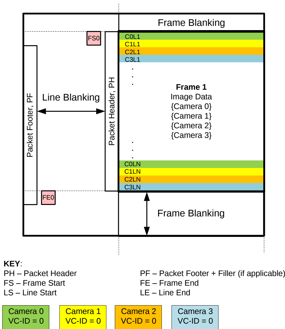
Figure 31. Line-Interleave Format
