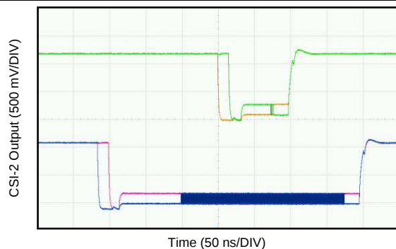
Figure 41. CSI-2 DATA and CLK Output
