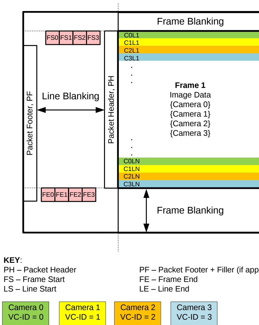
Figure 30. Basic Synchronized Format
