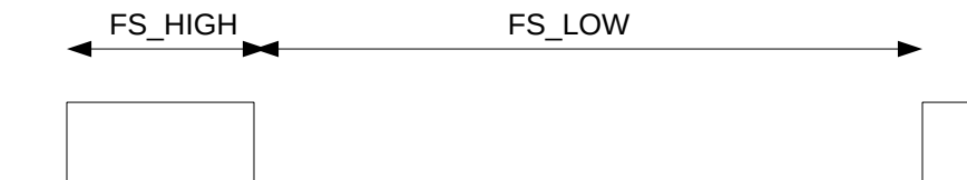
Figure 28. Internal FrameSync
