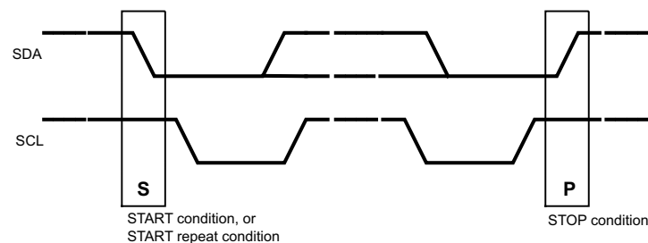
Figure 12. Start and Stop Conditions
