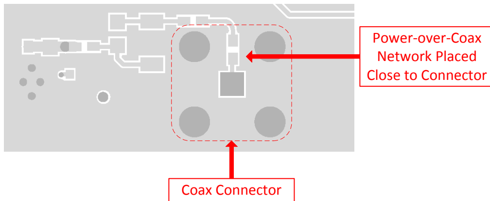
Figure 25. Power-over-Coax Layout
