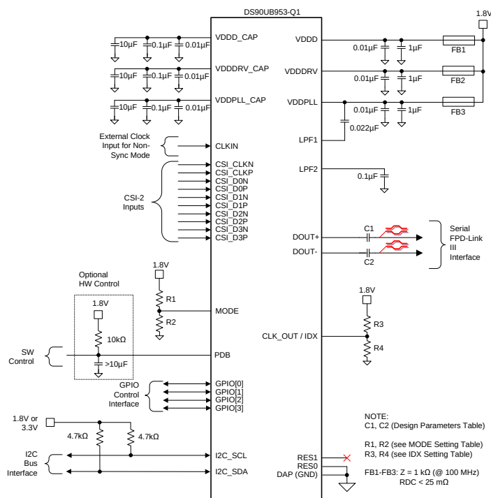
Figure 18. Typical Connection Diagram STP
