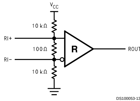
FIGURE 10. Terminated Input Fail-Safe Circuit
