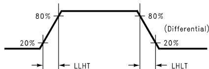
Figure 5. DS90C383B (Transmitter) LVDS Transition Times
