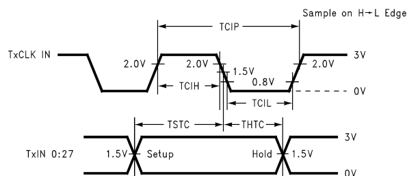
Figure 7. DS90C383B (Transmitter) Setup/Hold and High/Low Times (Falling Edge Strobe)
