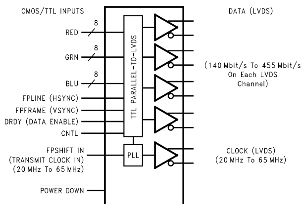
Figure 1. DS90C383B
