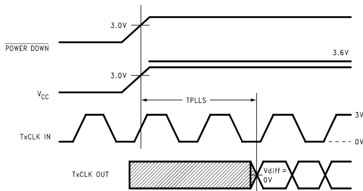
Figure 9. DS90C383B (Transmitter) Phase Lock Loop Set Time
