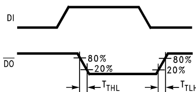
Figure 10. Driver Output Transition Time
