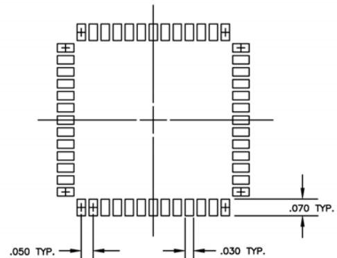
52 PIN QUAD (PLCC) SUGGESTED PAD LAYOUT
