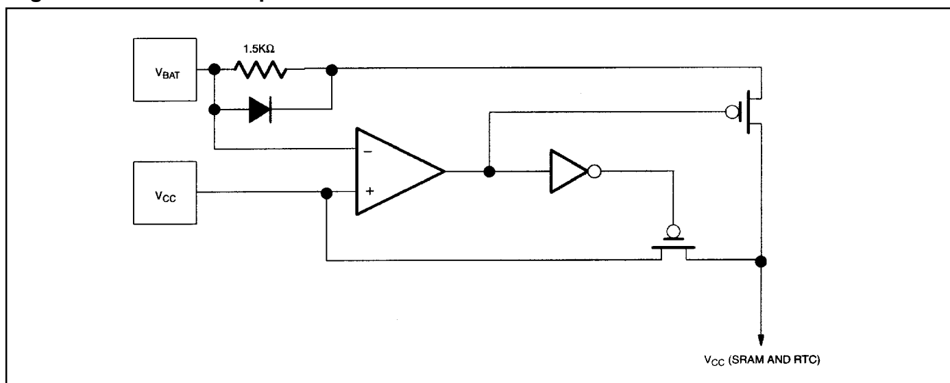
Figure 3. Internal Backup Circuit
