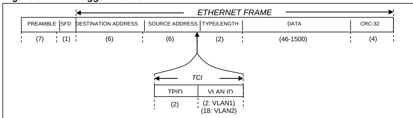
Figure 9. VLAN Tagged Frame
