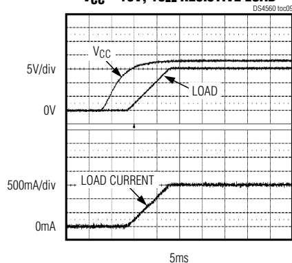
TURN-ON WAVEFORMS V_{CC} = 18V , 10 \Omega RESISTIVE LOAD
