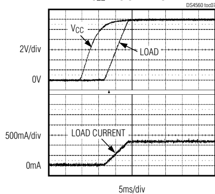
TURN-ON WAVEFORMS 10 \Omega RESISTIVE LOAD
