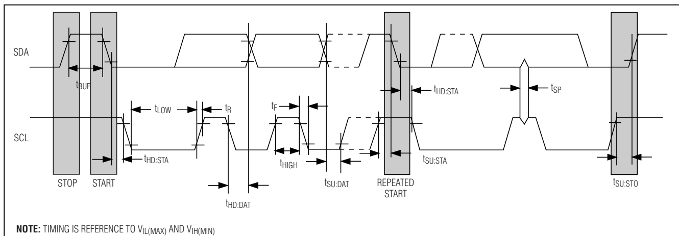
Figure 5. I²C Timing Diagram
