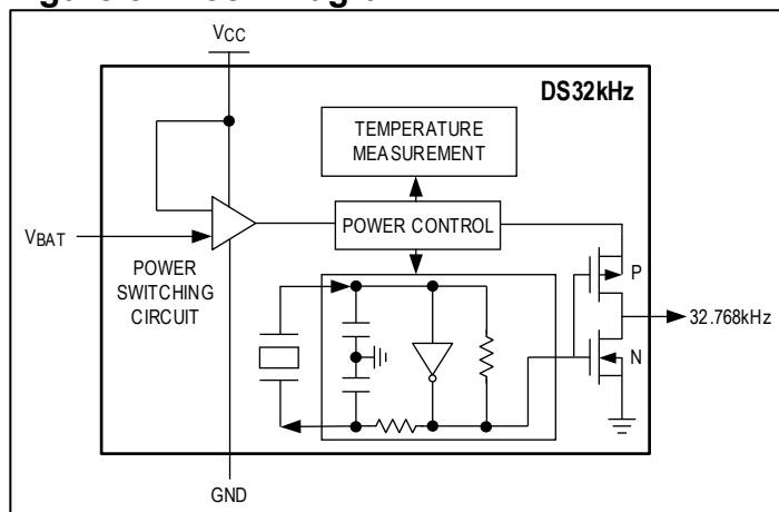
Figure 3. Block Diagram
