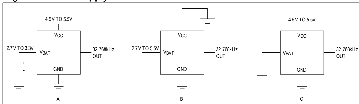
Figure 4. Power-Supply Connections
