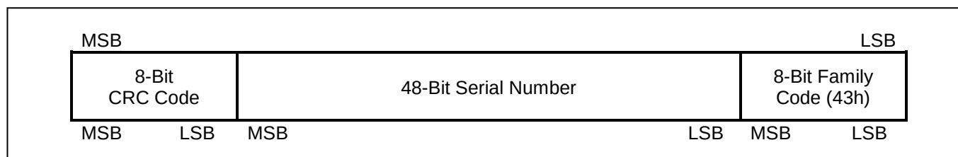
Figure 3. 64-Bit ROM
