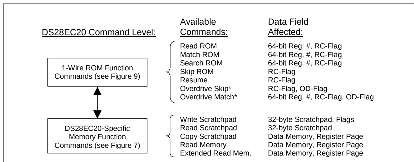
Figure 2. Hierarchical Structure for 1-Wire Protocol
