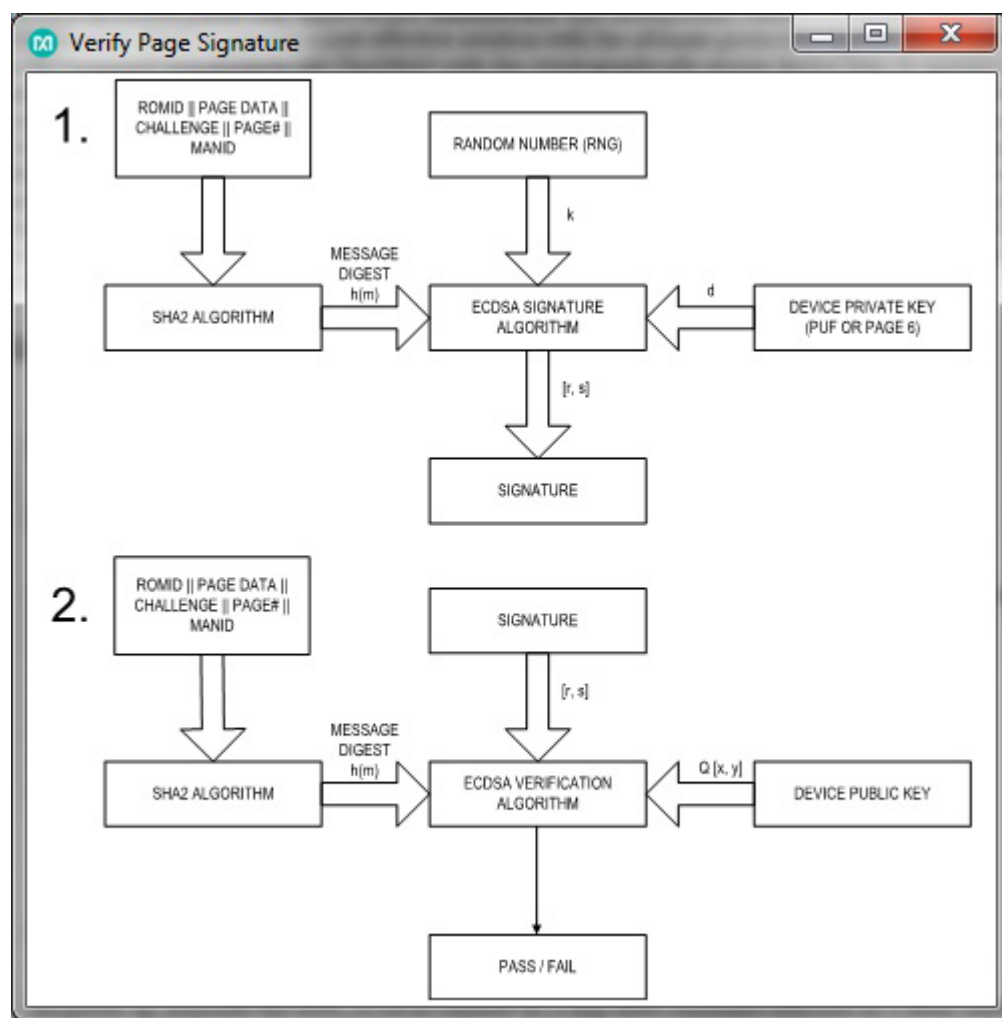
Figure 23. Ingredients Used to Verify the Signature
