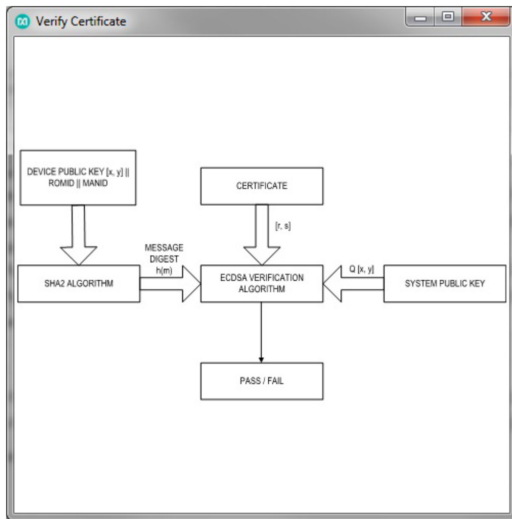
Figure 21. Ingredients Used to Verify the Certificate
