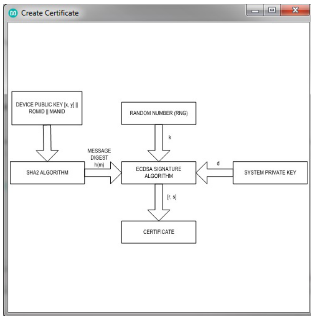
Figure 17. Ingredients Needed to Create the Certificate
