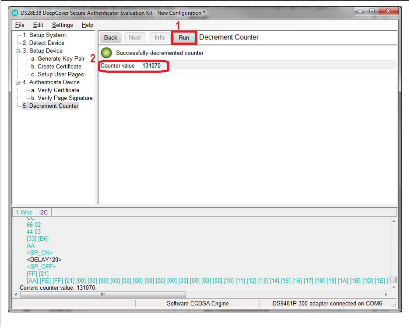
Figure 24. Decrement Counter
