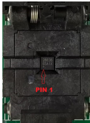
Figure 9. Orientation of the DS28E38 and DS2476 in the Burn-In Socket
