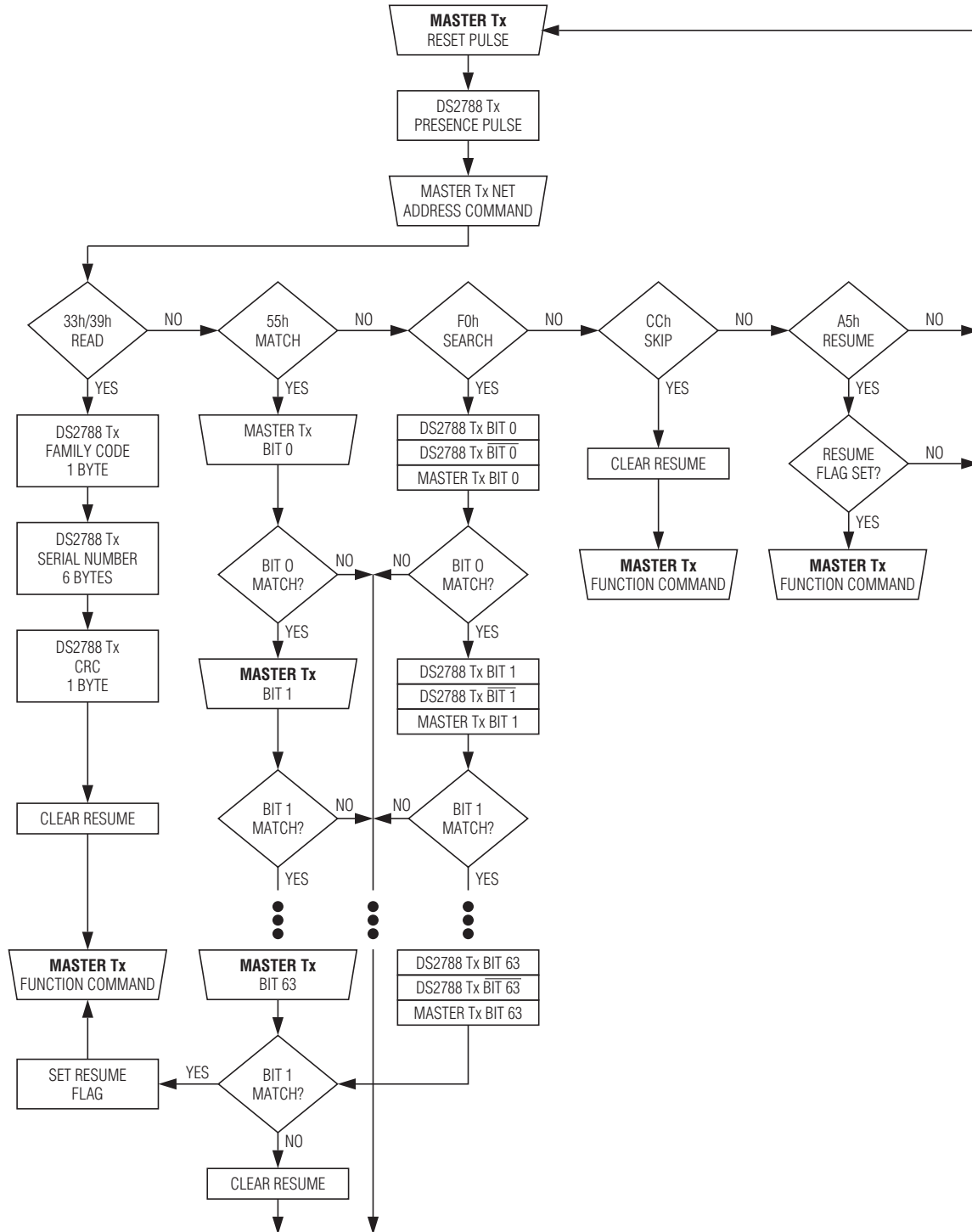
Figure 25. Net Address Command Flowchart
