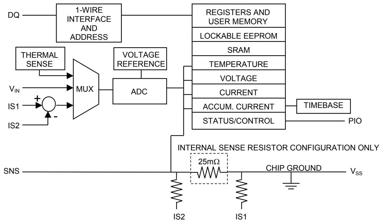
Figure 1. FUNCTIONAL DIAGRAM
