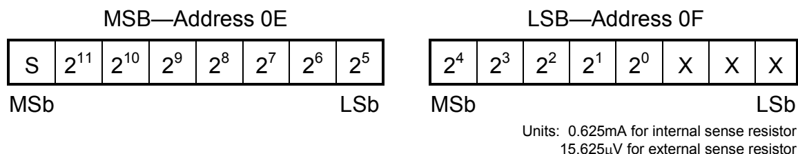
Figure 3. CURRENT REGISTER FORMAT
