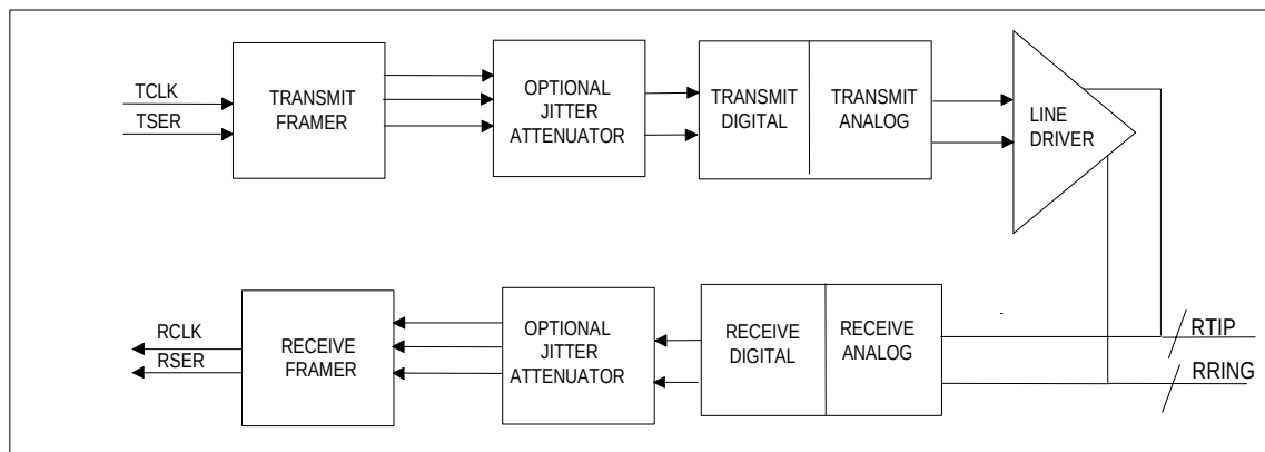
Figure 8-16. Analog Loopback
