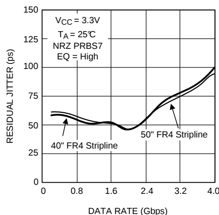
Figure 18. Residual Jitter as a Function of Data Rate, FR4 Stripline Length and EQ Level
