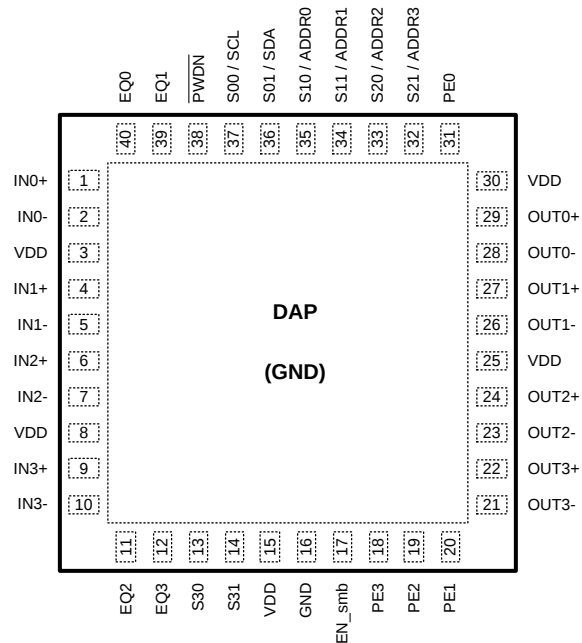
DS25CP104A / DS25CP114 Pin Diagram
