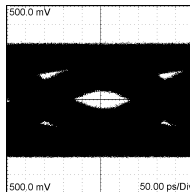
Figure 26. A 3.125 Gbps NRZ PRBS-23 without PE After 30" Differential FR-4 Stripline H: 50 ps / DIV, V: 100 mV / DIV
