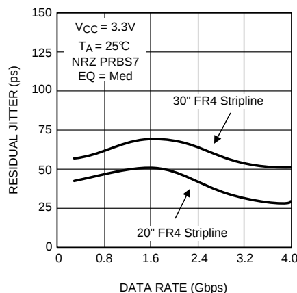
Figure 16. Residual Jitter as a Function of Data Rate, FR4 Stripline Length and EQ Level
