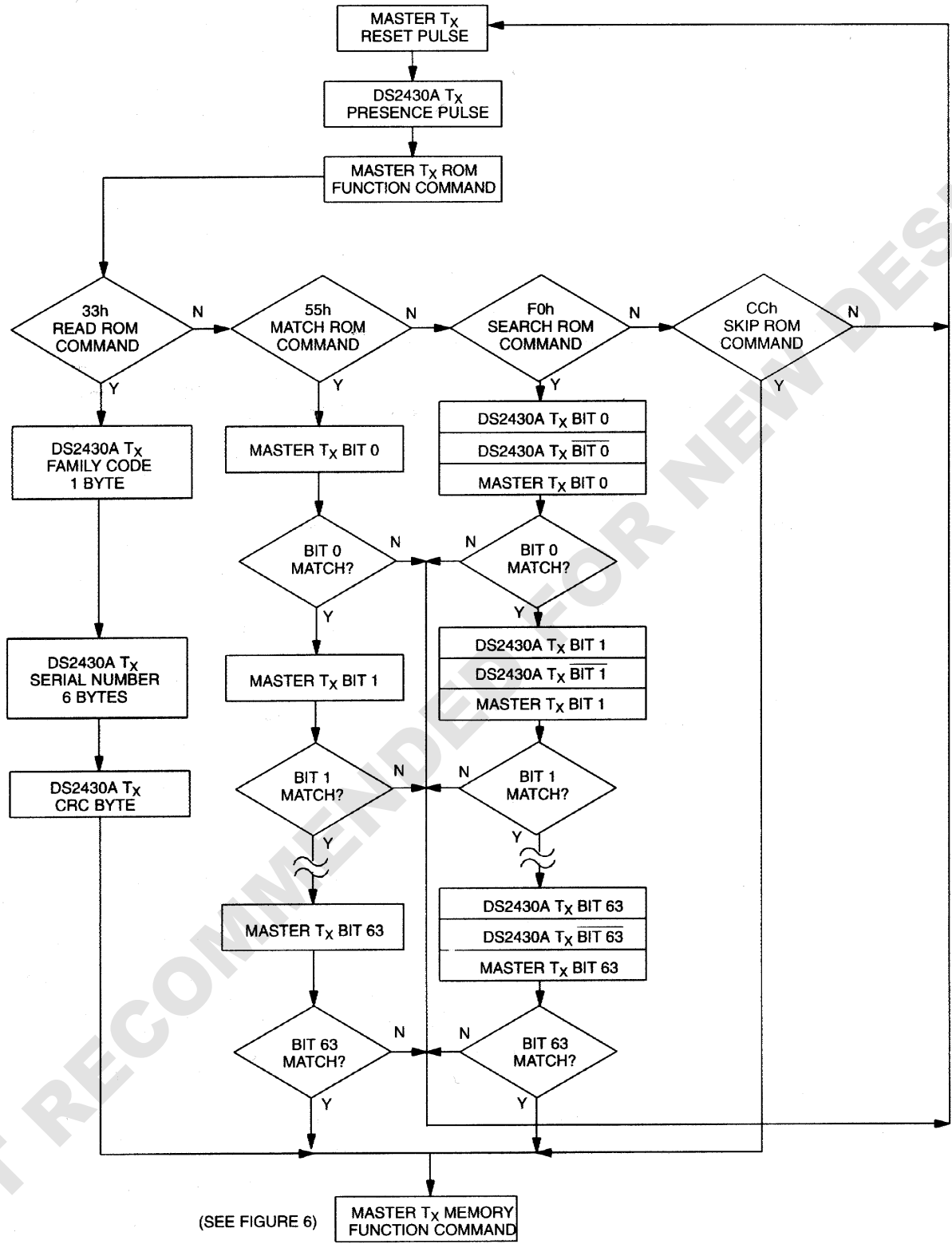
ROM FUNCTIONS FLOW CHART Figure 8
