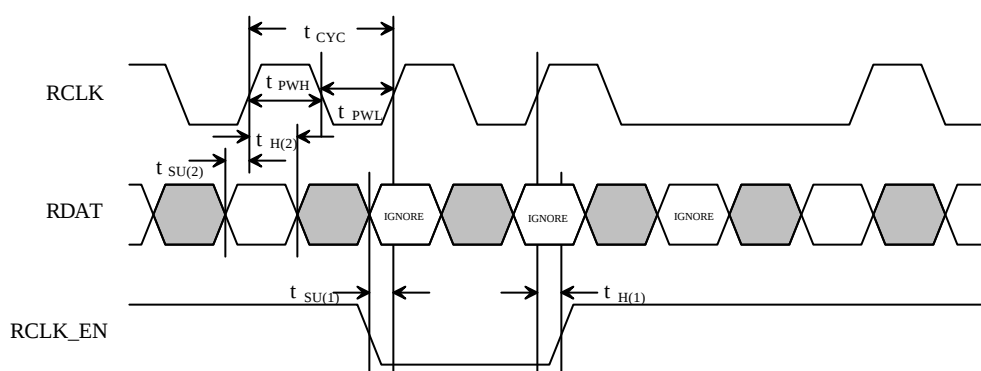
Figure 6-4. RECEIVE INTERFACE TIMING
