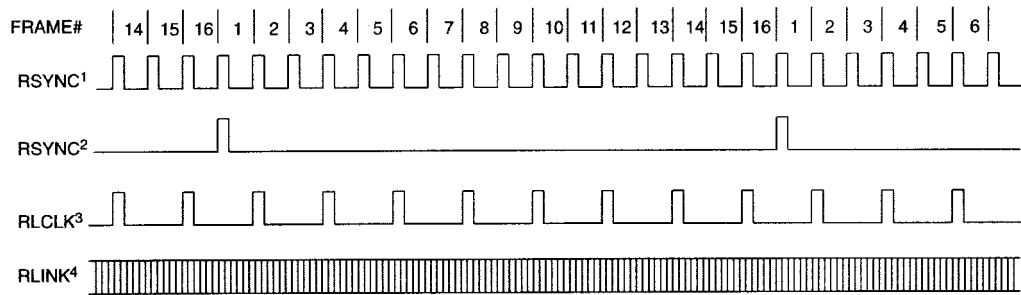
Figure 14-1. Receive Side Timing
