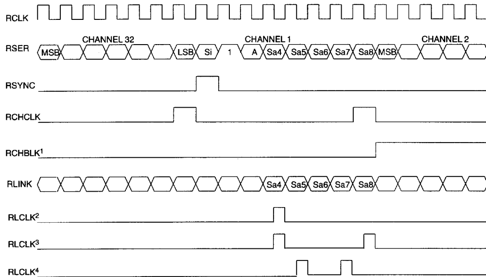
Figure 14-2. Receive Side Boundary Timing (with Elastic Stores Disabled)
