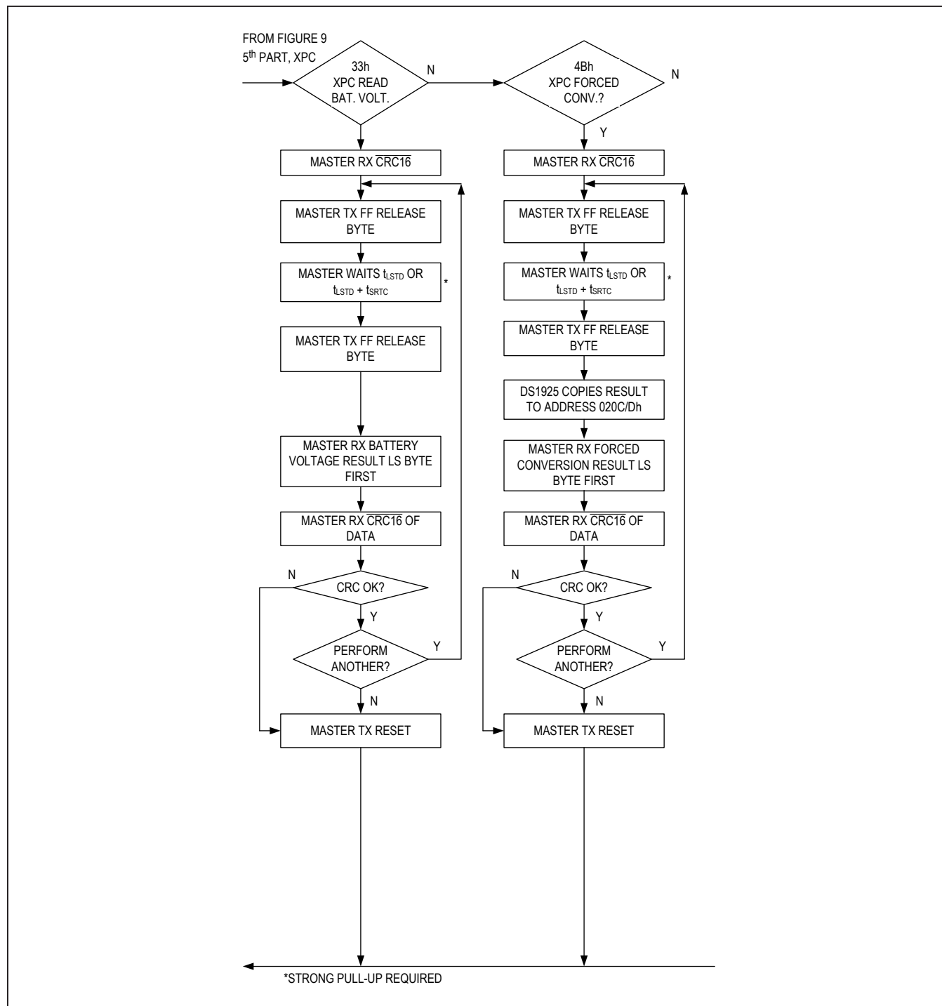
Figure 9f. Memory/Control Function Flowchart—XPC Subcommands Flowchart (continued)
