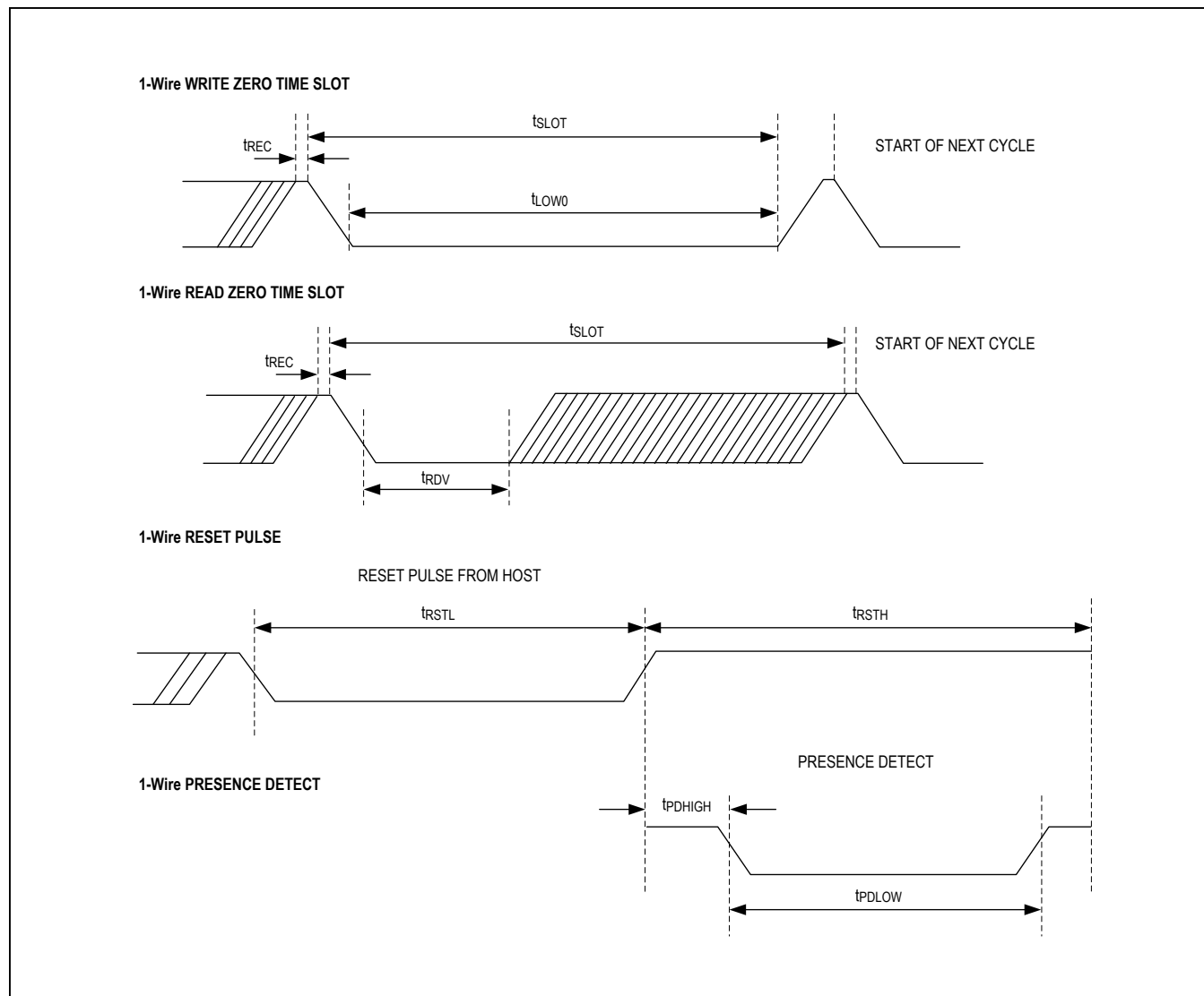
Figure 2. Timing Diagrams
