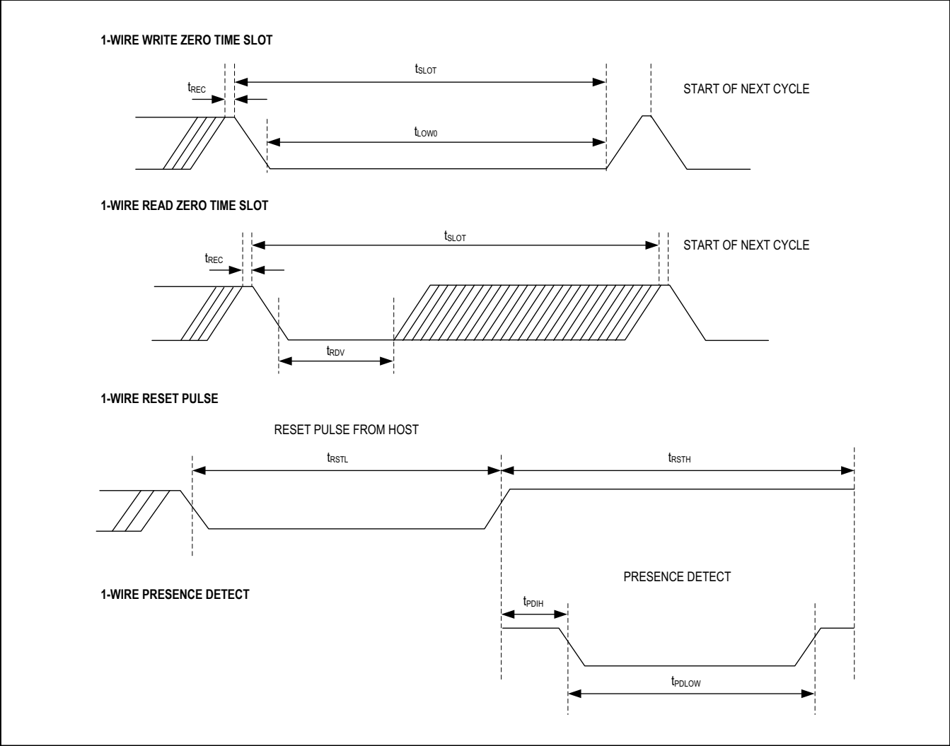
Figure 2. Timing Diagrams
