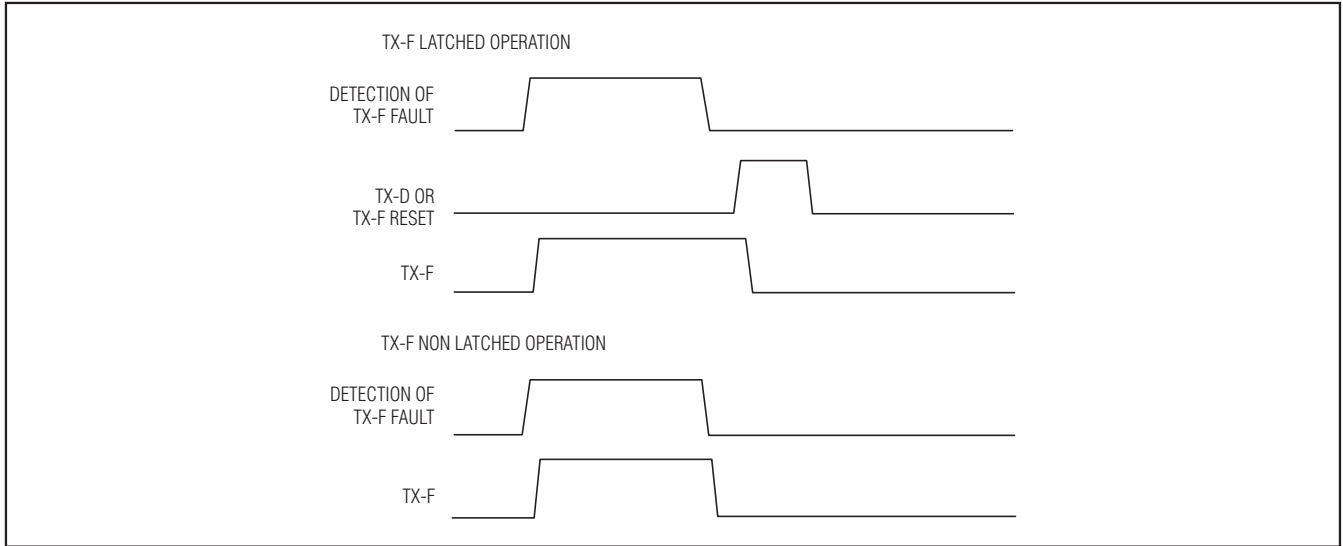
Figure 5. TX-F Timing
