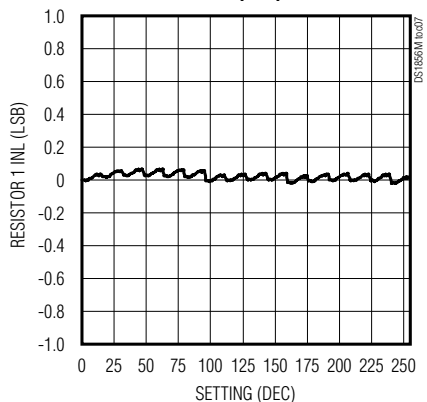
RESISTOR 1 INL (LSB) vs. SETTING
