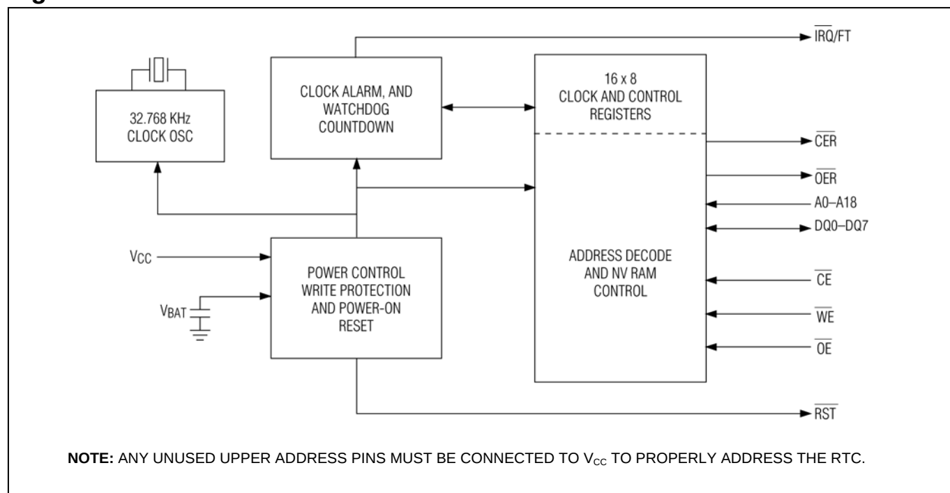
Figure 1. BLOCK DIAGRAM
