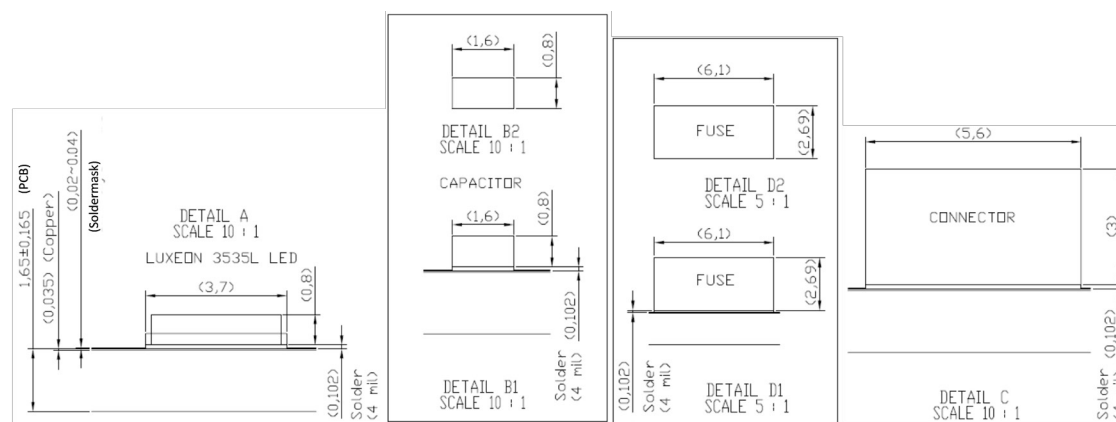
Figure 6: Mechanical dimensions for L202 – xxxx033C30000, component profiles.
