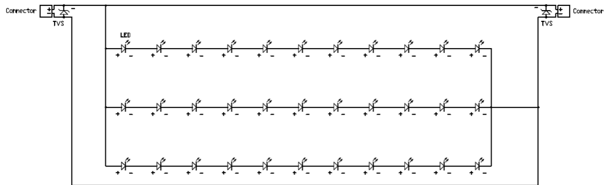
Figure 13: Electrical circuit diagram for L202 – xxxx033C30001.
