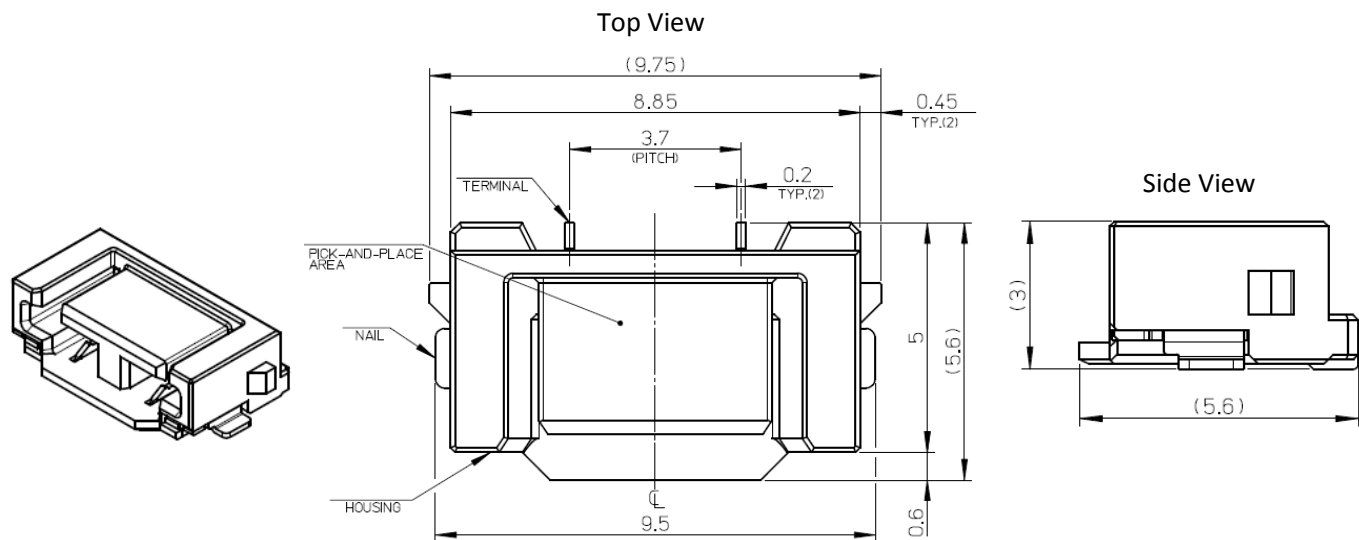
Figure 7: Mechanical dimensions for Molex (snap-together) connectors for L202 - xxxx033C30000.
