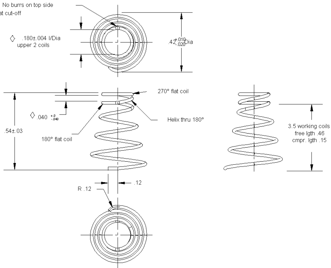
Diagram 2. DS1402D-010
