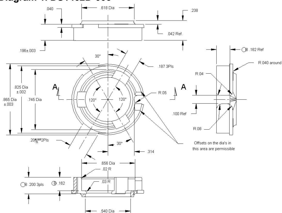
Diagram 1. DS1402D-003
