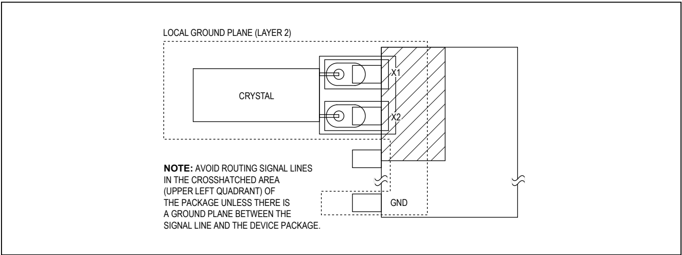
Figure 7. Layout Example
