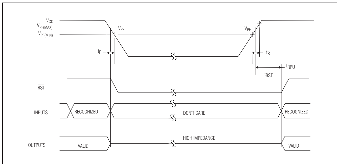
Figure 1. Power-Up/Down Timing
