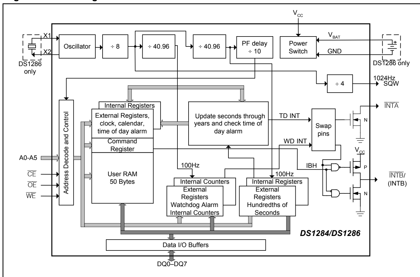
Figure 1. Block Diagram
