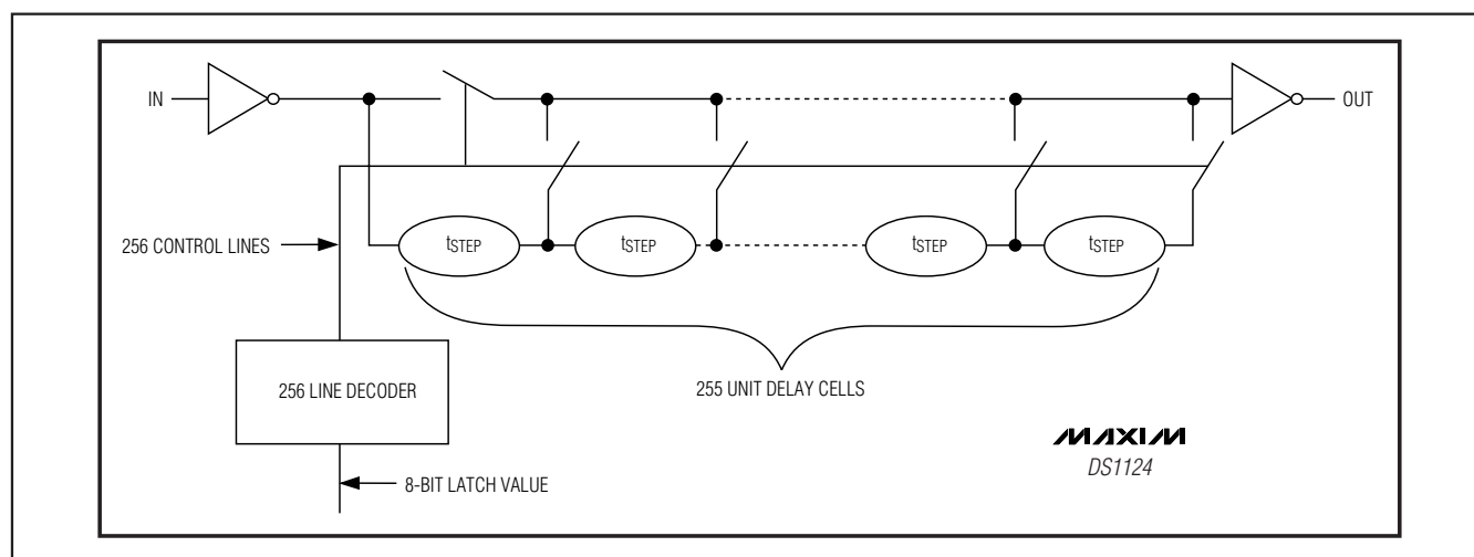
Figure 2. Conceptual Design
