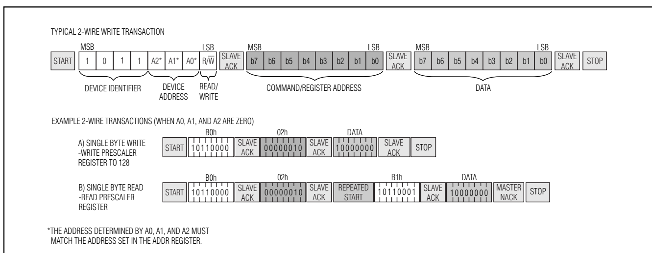
Figure 6. 2-Wire Transactions
