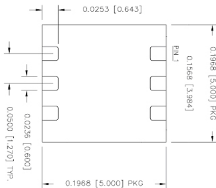
Figure 3: Recommended PCB layout to accommodate CBC012 package
