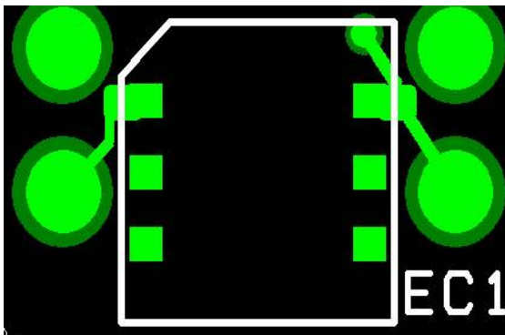
Figure 2: Proper PCB traces, precluding the formation of a parasitic leakage path.
