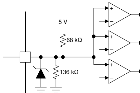
Figure 18. Quad-Level Input
