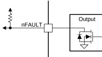
Figure 17. nFAULT Pin
