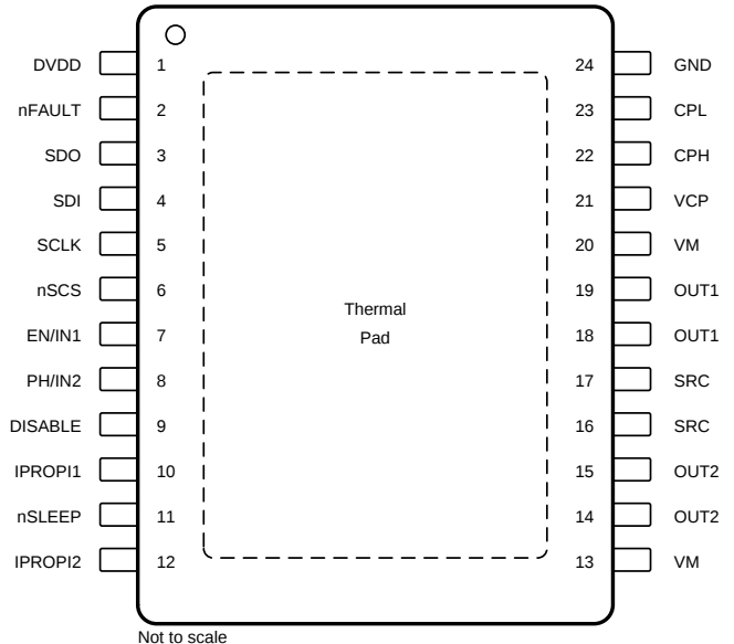
DRV8873S-Q1 PWP PowerPAD Package 24-Pin HTSSOP Top View
