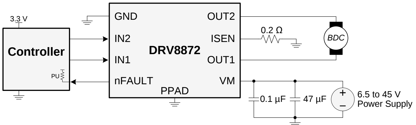
Figure 7. Typical Connections
