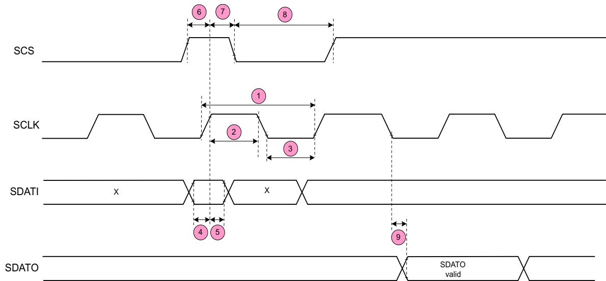
Figure 1. SPI Timing
