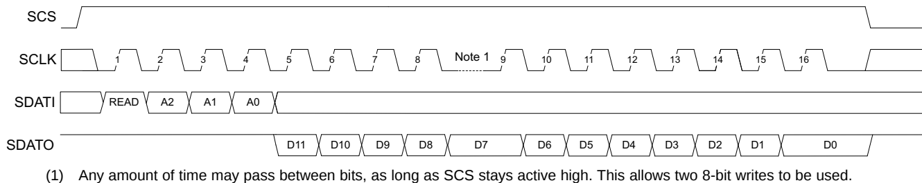
Figure 18. Read Operation
