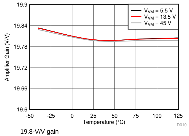
Figure 12. Amplifier Gain
