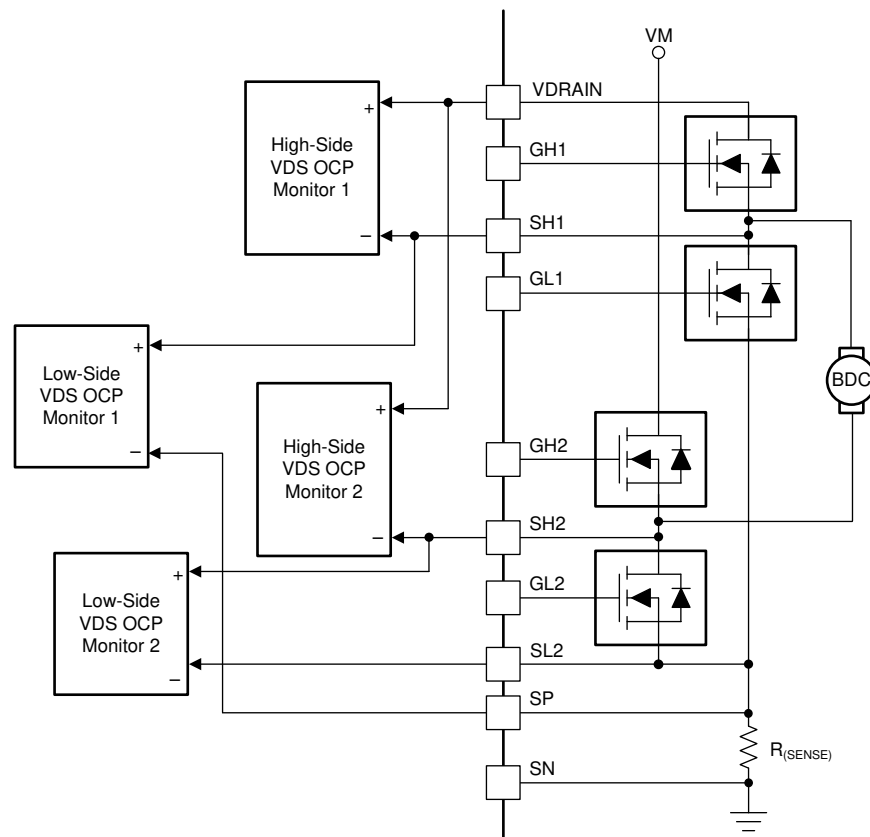
Figure 41. V_{DS(OC)} Block Diagram
