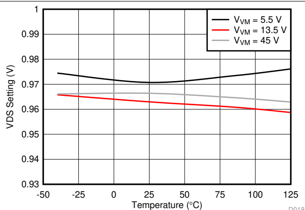
Figure 18. OCP Threshold Voltage
