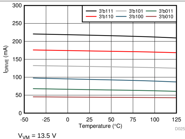
Figure 27. Low-Side Source Current
