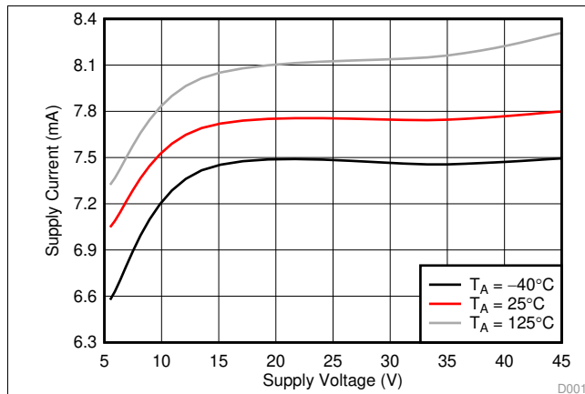
Figure 3. Supply Current vs Supply Voltage (VM)
