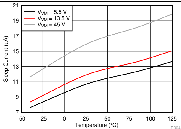
Figure 6. Sleep Current vs Temperature
