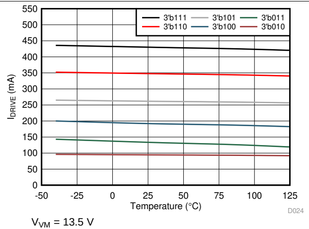
Figure 26. High-Side Sink Current
