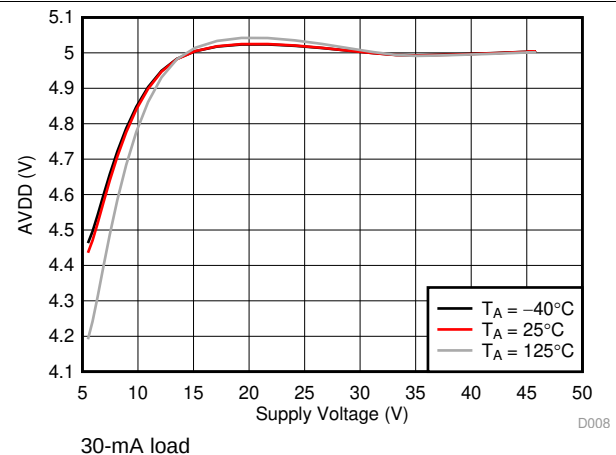
Figure 10. AVDD Regulator
