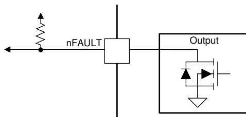
Figure 33. nFAULT Block Diagram
