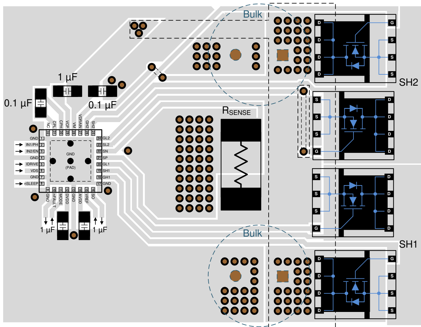
Figure 60. DRV8702-Q1 Layout Example
