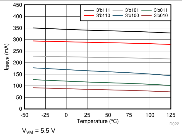
Figure 24. Low-Side Sink Current
