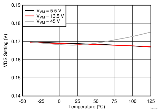
Figure 17. OCP Threshold Voltage
