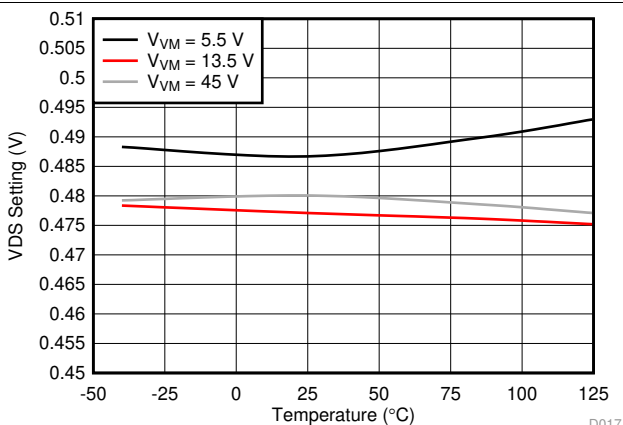
Figure 17. OCP Threshold Voltage
