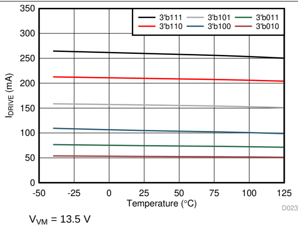
Figure 25. High-Side Source Current
