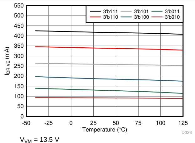
Figure 28. Low-Side Sink Current
