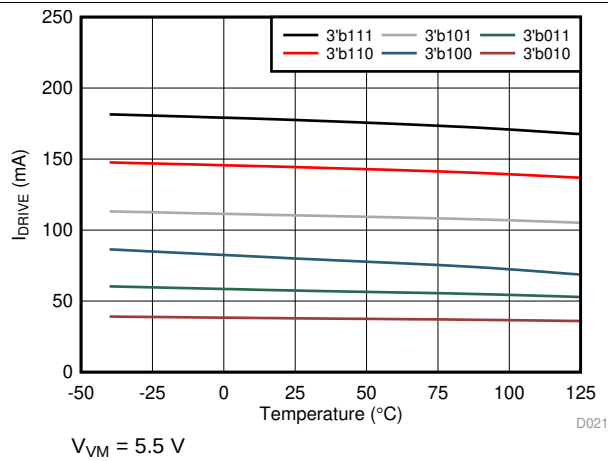
Figure 23. Low-Side Source Current
