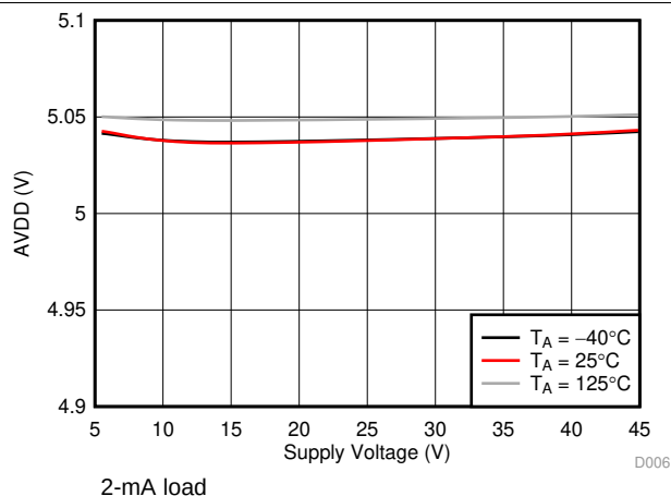
Figure 8. AVDD Regulator
