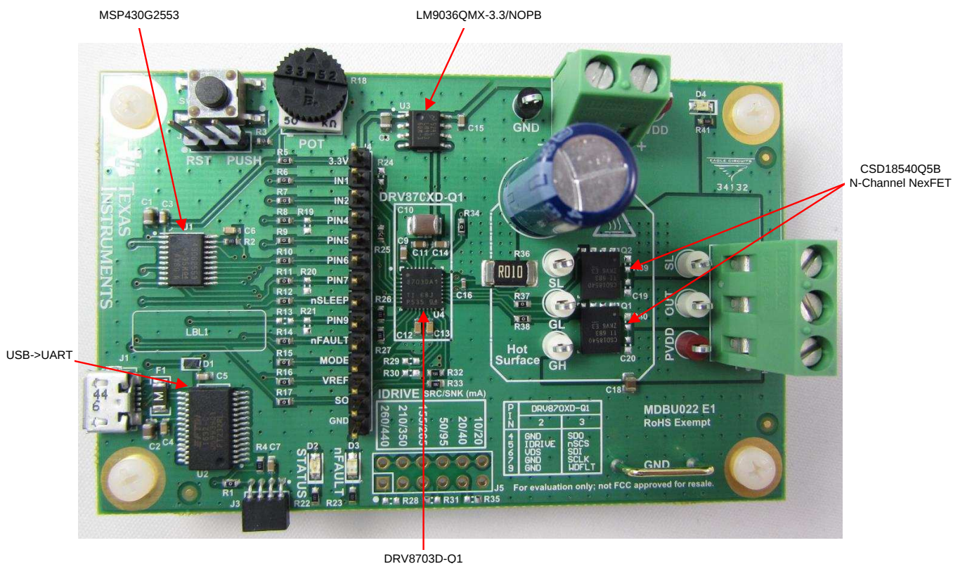
Figure 1. Board Components
