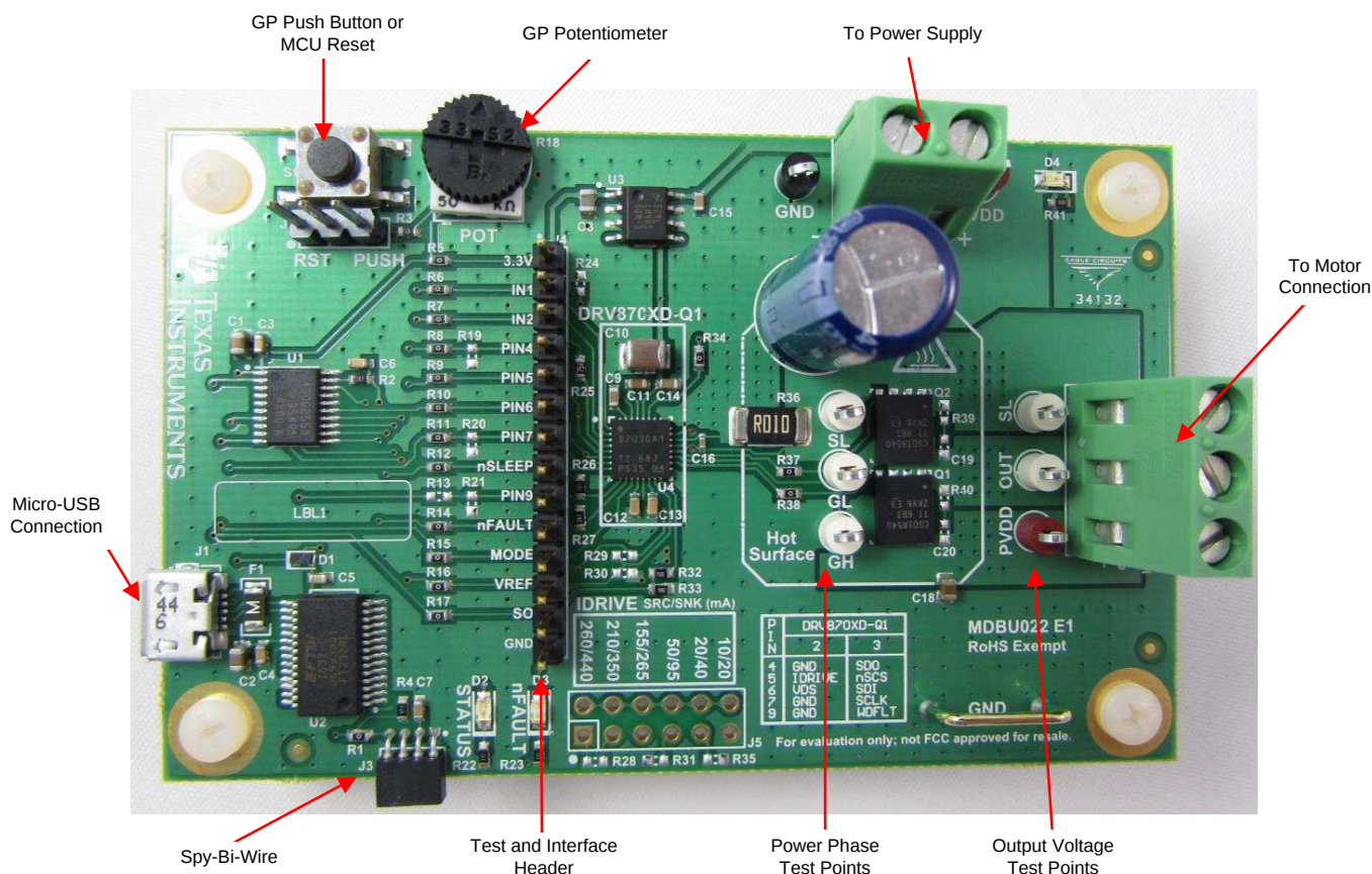
Figure 3. Board Jumpers and Test Points
