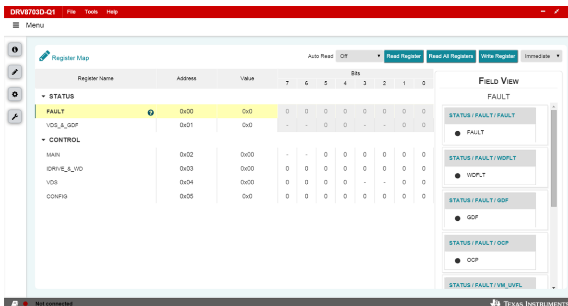
Figure 8. DRV8703D-Q1 EVM GUI (Register Page)
