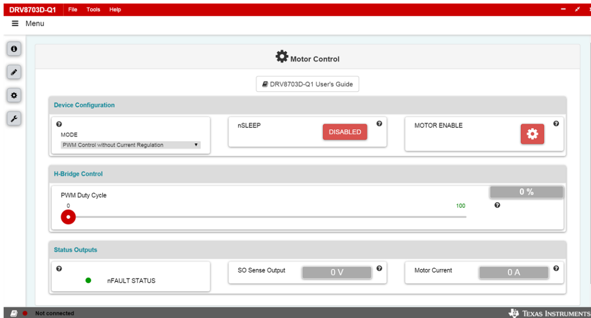
Figure 4. DRV8703D-Q1-EVM GUI (Motor Control Page)
